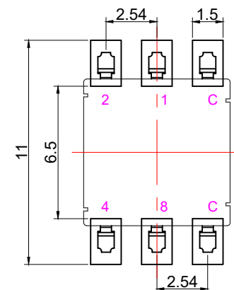
PCB LAYOUT
